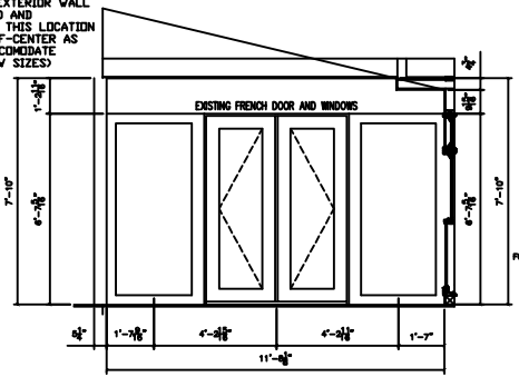
1 2 INTERIOR FACING SCREEN PORCH SCALE: 1/2" = 1'-0"
