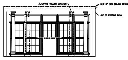
5 2 INTERIOR FACING YARD SCALE: 1/2" = 1'-0"
