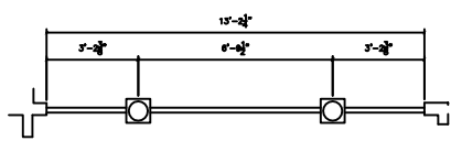
7 2 PROPOSED COLUMN SPACING SCALE: 1/2" = 1'-0"
