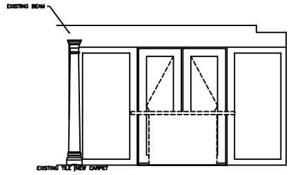
4 2 INTERIOR FACING SCREEN PORCH SCALE: 1/2" = 1'-0"
