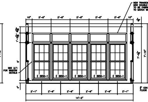
2 2 INTERIOR FACING YARD SCALE: 1/2" = 1'-0"
